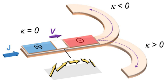
Fig. 9. Chiral DW in a ferromagnetic track traveling through a curvature speeds up or slows down depending on the sign of the curvature ( \kappa ).
