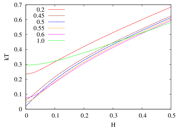
Figure 10. (Colour online) Temperature in dependence on the applied magnetic field for an isentropic cooling with fixed entropy S/N = 0.5 for spin s = 1/2 and N = 36 and various values of J_2 (given in the legend). Corresponding data for N = 20 (not shown) demonstrate that finite-size effects are small.
