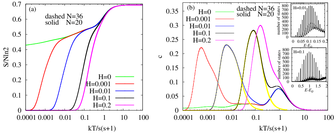
Figure 6. (Colour online) (a) Scaled entropy s(T)/N \ln(2s + 1) per site for periodic chains of N = 20 (ED) and 36 (FTLM) sites with J_1 = -1 , J_2 = 1/2 and spin s = 1/2 for various magnetic fields H . (Note that the curves for N = 20 and N = 36 coincide, i.e., the dashed lines are practically not visible.) (b) Main panel: Influence of the magnetic field H on the specific heat c(T) per site for periodic chains of N = 20 (ED — solid) and N = 36 (FTLM — dashed) sites with J_1 = -1 , J_2 = 1/2 and spin s = 1/2 . (Note that the curves for N = 20 and N = 36 perfectly coincide, i.e., the dashed lines are practically not seen.) The broad yellow curves are calculated using a restricted set of energies to determine the specific heat, namely E < E_0 + 0.15 ( E < E_0 + 1.5 ) for H = 0.01 ( H = 0.1 ). Inset: Density for states for H = 0.01 and H = 0.1 shown for that energy region relevant for the extra low-temperature maximum in c(T) presented in the main panel.
