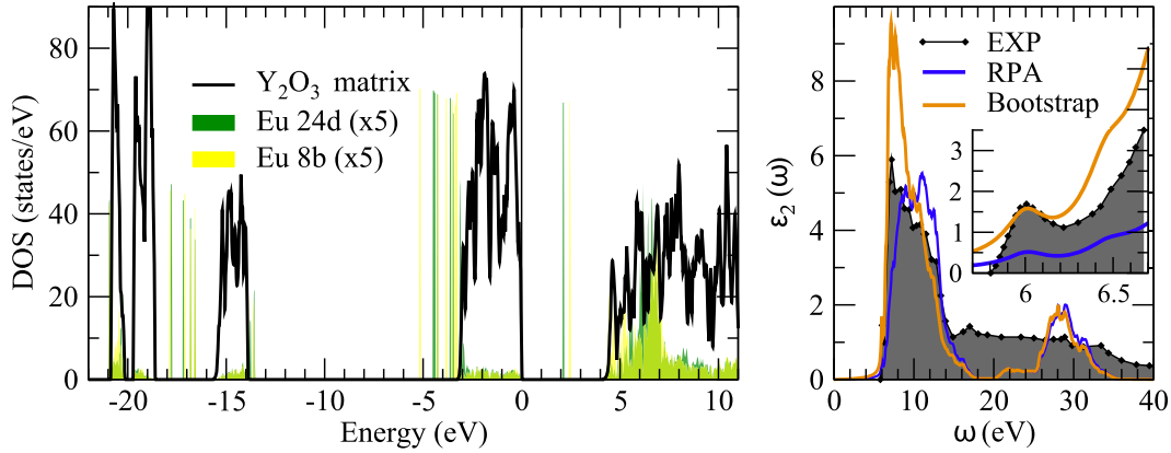
Figure 2. Left: density of electronic states of \text{Y}_2\text{O}_3 (black) and contribution from Eu impurities in the 24d (green) and 8b (yellow) sites. Right: the RPA and bootstrap-TDDFT [23, 25] absorption spectra for \text{Y}_2\text{O}_3 in comparison with the experimental results from reference [22].
