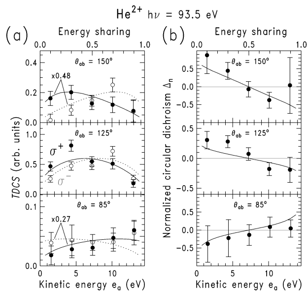
FIG. 4. (a) The helium double photoionization TDCS versus kinetic energy sharing at h\nu = 93.5 \text{ eV} for three different relative emission angles \theta_{ab} of the two electrons. The circles correspond to measurements with negative (open) and positive (full) helicity of the circularly polarized radiation. The solid and dotted curves are our theoretical results arbitrarily scaled (as quoted) with respect to the experimental TDCS. (b) Normalized circular dichroism for the three corresponding relative emission angles. The full curves represent our theoretical results. Note the different scaling of the three plots in (a) and (b), respectively.
