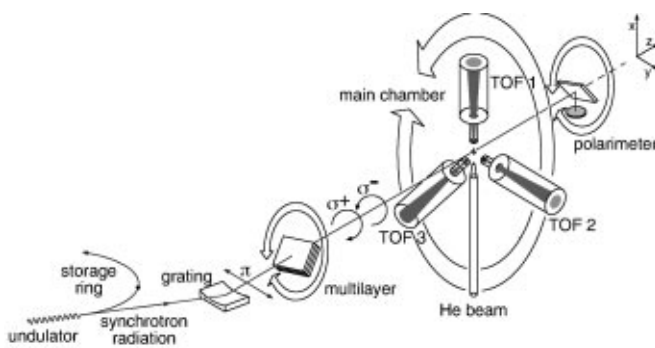
FIG. 2. Schematic drawing of the experimental setup. Three TOF electron analyzers are mounted in a plane perpendicular to the incoming photon beam. The linear polarized radiation is transformed into circular polarized radiation by a transmission multilayer positioned at the entrance of the vacuum chamber. The helicity of the radiation can be switched using appropriate polar angles for the multilayer.
