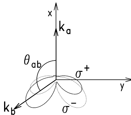
FIG. 1. Schematic drawing of the experimental geometry. The directions of emission of the two electrons given by \mathbf{k}_a and \mathbf{k}_b are lying in a plane perpendicular to the propagation direction of the circularly polarized ionizing radiation which is pointing into the plane of the drawing. The relative angle between the two directions of emission is given by \theta_{ab} . A calculated TDCS for h\nu = 93.5 eV and E_a/E_b = 1/9 is shown for both helicities ( \sigma^+/\sigma^- ).
