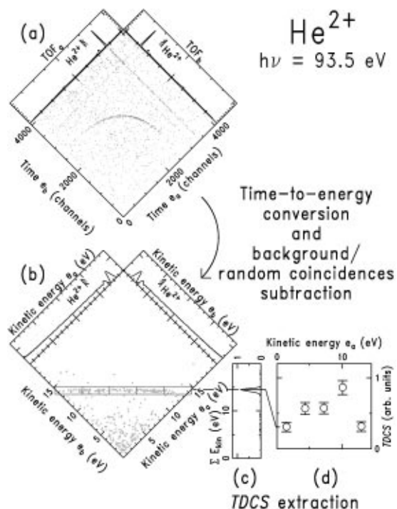
FIG. 3. Overview of the data analysis of the helium double photoionization electron spectra. (a) The noncoincident electron raw spectra of two TOF analyzers as well as the simultaneously recorded two dimensional raw coincidence spectrum of the corresponding analyzer pair. (b) The same spectra on kinetic energy scale and after subtraction of the background and random coincidence events, respectively. (c) The double ionization photoelectron spectrum, generated by plotting all coincidence events versus excess energy. (d) The TDCS intensity versus energy sharing.
