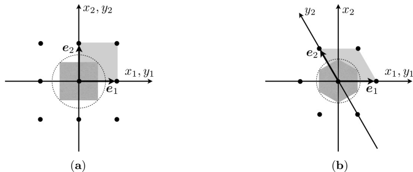
FIG. 1. Two-dimensional lattices ( \ell = 1 ): (a) the \mathbb{Z}^2 square lattice, (b) the A_2^* hexagonal lattice. The fundamental polytopes are shown in light grey, the WS cells are shown in dark grey and inscribed by the dashed circles of the covering radius. For general n , the basis vectors e_i for A_n^* define vertices of an equilateral n -simplex (see text after Eq. (2.10)).
