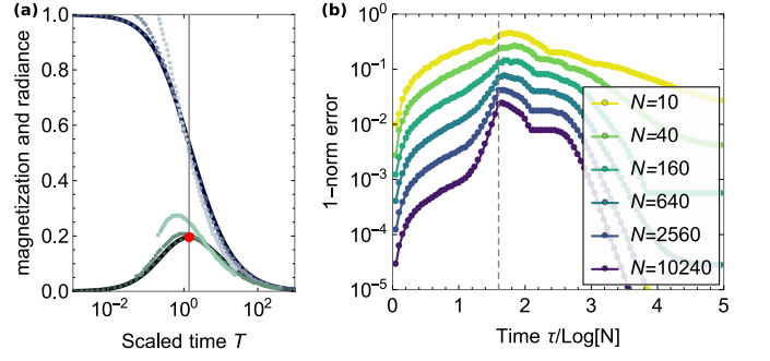
FIG. 1. (a) Magnetization \mu (blue, solid) and radiance \rho (green, solid) as defined in Eq. (18), together with numerical data for N = 5, 20, 1000 showing quick convergence. The largest radiance is \rho \approx 0.196 at T \approx 1.391 , marked with a red dot. (b) Numerical evaluation of the 1-norm error Eq. (14), which vanishes as N \rightarrow \infty by Theorem 1. The dashed line marks \tau_1 = 1.6 \log N .
