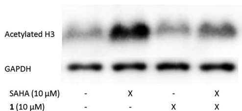
Fig. 2 Compound 1 decreases histone H3 acetylation levels in LNCaP cells. Cells were treated with 1 and the HDAC inhibitor suberoylanilide hydroxamic acid (SAHA) for 3 hours at the concentrations indicated. Extracts were probed with antibodies against acetylated histone H3 and GAPDH as a loading control. The SAHA induced hyperacetylation is suppressed by compound 1.
