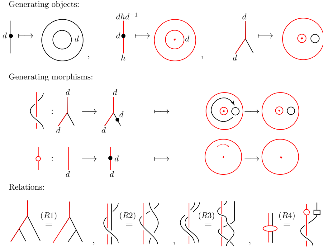
Figure 12: Generating operations and relations for D\text{-fBr}^1 and their image under the equivalence D\text{-fBr}^1 \xrightarrow{\cong} \Pi_1(D\text{-fE}_2^1) . Notice that we did not depict the relations related to the D -action. The d -labels on the disk for the first two generating objects mean that the map to BD is the loop d in radial direction. In D\text{-Man}_2 this embedding is isomorphic to the identity embedding equipped with the homotopy corresponding to d . If we ignore the D -labels, we get generators and relations of \text{fBr}^1 . If we furthermore drop the second generating morphism as well as relation (R4), we get a combinatorial model for \text{E}_2^1 .
