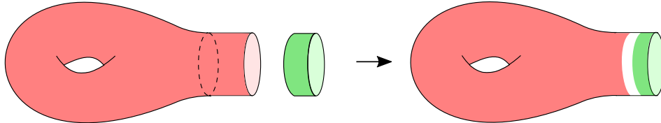
Figure 3: The map which induces the right \int_{M_0} \mathcal{A} -module structure on \int_{M_-} \mathcal{A} . Here, the green collar depicts the manifold N \times (-1, 1) .
