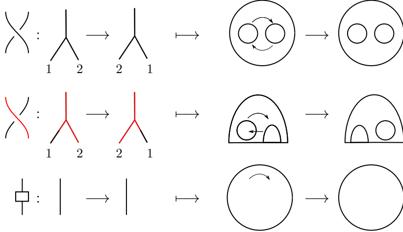
Figure 11: Generating operations for \mathbf{fPeBr} and their image under the equivalence \mathbf{fPeBr} \xrightarrow{\cong} \Pi_1(\mathbf{fSC}) . The arrows indicate the paths in the space of embeddings. If we ignore the last generating morphism, we recover the generators of \mathbf{PeBr} .
