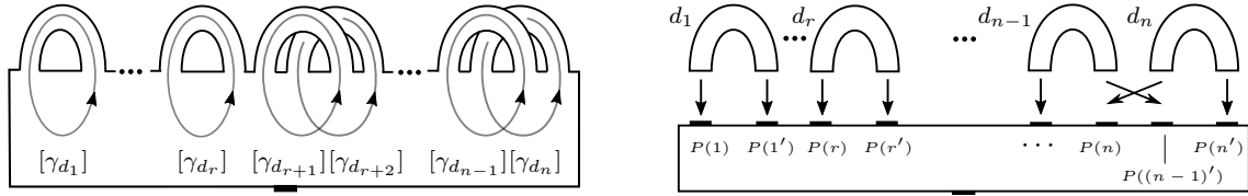
(a) Generators of the homotopy group \pi_1(\Sigma) . (b) Gluing a surface from a decorated gluing pattern.
