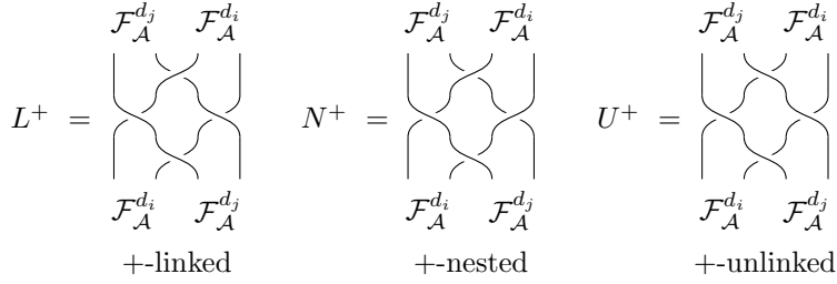
Figure 6: Definition of crossing-morphisms L^+, N^+, U^+ : \mathcal{F}_A^{d_i} \otimes \mathcal{F}_A^{d_j} \rightarrow \mathcal{F}_A^{d_j} \otimes \mathcal{F}_A^{d_i} for positively linked, nested and unlinked decorated discs. Notice that we read the diagrams from bottom to top.
