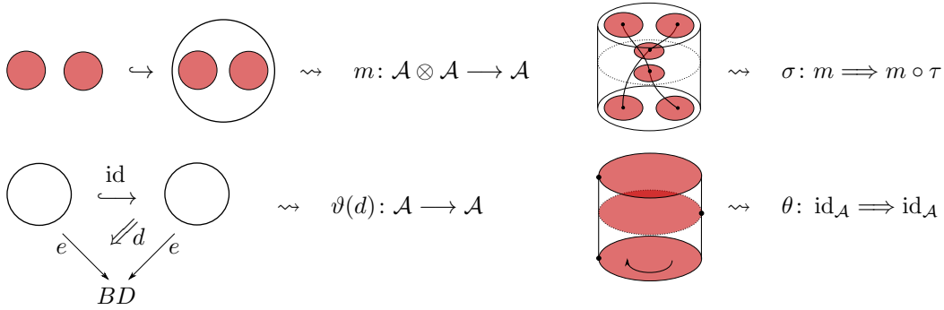
Figure 1: First row: Disk embeddings (or isotopies thereof) in \text{Disk}_2^* that give rise to the multiplication m and the braiding \sigma in the E_2 -algebra \mathcal{A} . Here \tau: A \otimes A \rightarrow A \otimes A denotes the braiding in \mathcal{V} . Second row: On the right, the additional operation in the oriented case given by a loop in the space of disk embeddings in \text{Disk}_2^{SO(2)} , rotating the disk by 2\pi . Together with the operations in the first row, this endows \mathcal{A} with the structure of a framed E_2 -algebra. On the left, the additional operation in the D -decorated oriented case, given by the identity disk embedding in \text{Disk}_2^{SO(2) \times D} with homotopy d: \text{id}^*(e) \Rightarrow e , inducing an automorphism of \mathcal{A} for each d \in D , i.e. a D -action on \mathcal{A} .
