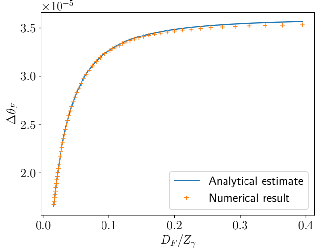
FIG. 5. Phase difference for a short, perfectly synchronized 10 keV x-ray pulse due to vacuum birefringence in a FF pulse with \lambda_F = 1 \mu\text{m} , \hat{w}_F = 3 \mu\text{m} , \mathcal{E}_F = 1000 \text{ J} , and P_F = 15 \text{ TW} . The interaction length is D_F = 1 \text{ cm} . The phase difference is plotted as a function of D_F/Z_\gamma for the numerical solution [solving Eqs. (D5) and (D6) for both polarizations] and the analytical approximation in Eq. (E3). The range of D_F/Z_\gamma values corresponds to spot sizes \hat{w}_\gamma \in (1, 5) \mu\text{m} .
