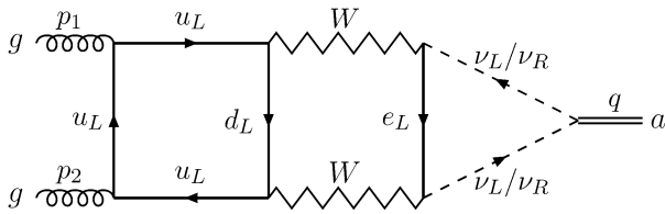
Fig. 2 Axion–gluon–gluon effective vertex
