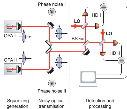
FIG. 2 (color online). Schematic experimental setup. Two amplitude-squeezed beams were produced by two length-controlled OPA cavities. Quasirandom band-limited Gaussian white phase noise is applied to both squeezed beams to mimic phase noise in optical transmission channels. The two beams are subsequently overlapped at a 50/50 beam splitter ( BS_{PUR} ). Time series of quadrature values for both beam splitter outputs were recorded using balanced homodyne detection (HD) and a data acquisition system. OPA: optical parametric amplifier; LO: local oscillator; \blacksquare : piezo-electric transducer.
