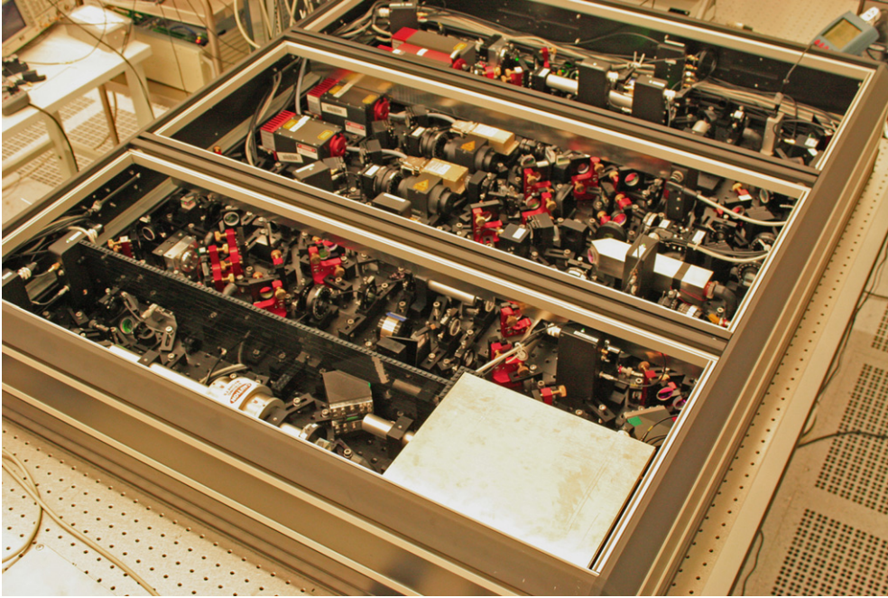
Figure 2. Photograph of the GEO 600 squeezed light source. The breadboard dimensions are 135 cm \times 113 cm. The three Nd:YAG lasers are located on the upper left, at the bottom left the squeezing resonator and on the bottom right the homodyne detector with its covering box is shown. The total weight of the complete system is approximately 130 kg.
