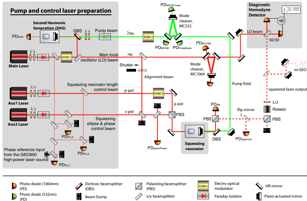
Figure 1. Schematic of the complete optical setup of the GEO 600 squeezed light source including control lasers and diagnostic tools. Squeezed states of light at audio-band Fourier frequencies around the carrier frequency \omega_0 are produced inside a nonlinear squeezing resonator via parametric down conversion. The squeezing resonator contains a birefringent nonlinear crystal that is pumped with a green laser beam at 532 nm. Two auxiliary laser beams are also focussed into the crystal and serve as control beams for piezo-electric length stabilization of the cavity and the green pump phase. A balanced homodyne detector was used to characterize the squeezed light output.
