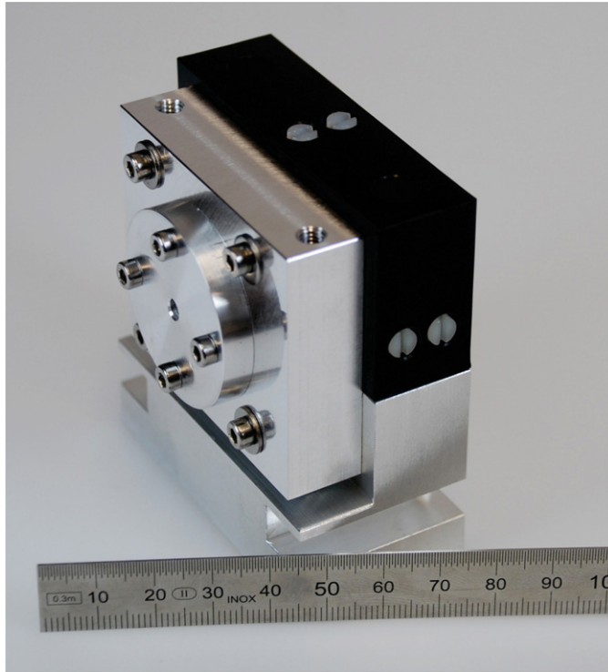
Figure 3. Photograph showing the housing of the nonlinear squeezing resonator. Nonlinear crystal, peltier and piezo-elements as well as the out-coupling mirror are embedded in a compact quasi-monolithic design for a high intrinsic mechanical stability.
