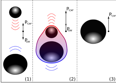
FIG. 1 (color online). Cartoon of the generation of the antikick in the head-on collision of two unequal-mass Schwarzschild BHs. Initially the smaller BH moves faster and linear momentum is radiated mostly downwards, thus leading to an upwards recoil of the system [stage (1)]. At the merger the curvature is higher in the upper hemisphere of the distorted BH (cf. shading) and linear momentum is radiated mostly upwards leading to the antikick [stage (2)]. The BH decelerates till a uniform curvature is restored on the horizon [stage (3)].
