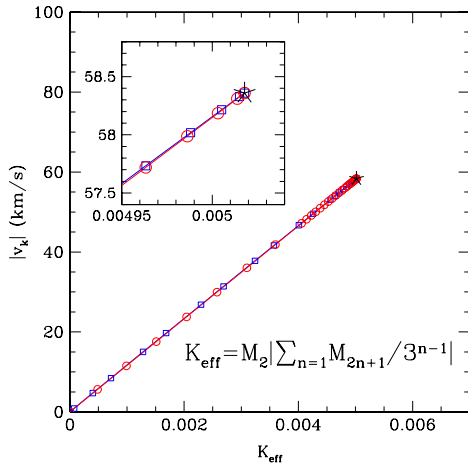
FIG. 4 (color online). Recoil velocity shown as a function of the effective curvature. In contrast with Fig. 3, which uses the same symbols employed here, the relation between the curvature and the recoil is now injective.
