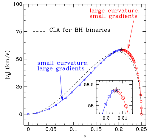
FIG. 3 (color online). Recoil velocity shown as a function of the symmetric mass ratio \nu when w = -0.425 , with the dashed line refers to the antikick from the inspiral of nonspinning binaries in the CLA [17]. Note that the curve can be thought of as being composed of two different branches.
