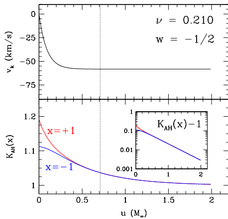
FIG. 2 (color online). Typical evolution of a RT spacetime. Shown in the lower panel is the evolution of the curvature K_{\text{AH}} at the north ( x = 1 ) and south pole ( x = -1 ). Shown in the upper panel is the evolution of the recoil, which stops decreasing when the curvature difference is erased by the radiation (dotted line).
