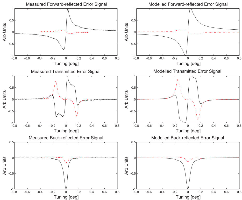
Figure 2. Normalized RF power for each output port: forward-reflect (top), transmitted (middle), and back-reflect (bottom). The measured data and modelled predictions of the length sensing signals are presented on the left- and right-hand sides respectively. The solid (black) trace indicates in-phase measurements, and the dashed (red) trace indicates quadrature-phase. The absolute scaling between modelled forward-reflect, transmitted, and back-reflect ports is 163:1:2.
