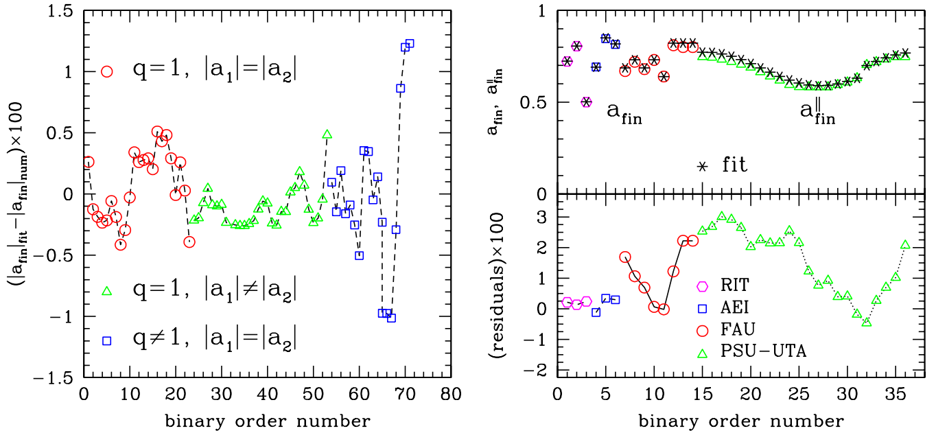
FIG. 1 (color online). Left panel: rescaled residual for aligned binaries. The circles refer to equal-mass, equal-spin binaries presented in Refs. [11–13,20–22], triangles to equal-mass, unequal-spin binaries presented in Refs. [11,21], and squares to unequal-mass, equal-spin binaries presented in Refs. [13,20–22]. Here and in the right panel the “binary order number” is just a dummy index labelling the different configurations. Right panel: the top part reports with asterisks the final spins computed for misaligned binaries. Hexagons refer to data from Ref. [8] (labeled “RIT”), squares to the data Table I (labeled “AEI”), circles to data from Ref. [23] (labeled “FAU”), and triangles to data from Ref. [24] (labeled “PSU-UTA”). Note that these latter data points refer to the aligned component a_{\text{fin}}^{\parallel} since this is the only component available from Ref. [24]. The bottom part of this panel shows instead the rescaled residuals for these misaligned binaries.
