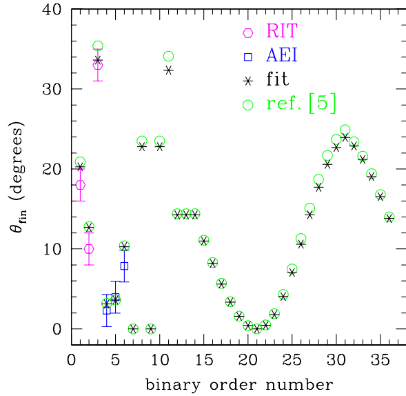
FIG. 2 (color online). Using the same data (and convention for the symbols) as in the right panel of Fig. 1, we here report the angle between the final spin vector and the initial orbital angular momentum \theta_{\text{fin}} . Shown instead with asterisks and circles are the values predicted for the numerical data (as taken from Refs. [8,23,24] and from Table I) by our analytic fit (asterisks) and by the point-particle approach suggested in Ref. [5] (circles).
