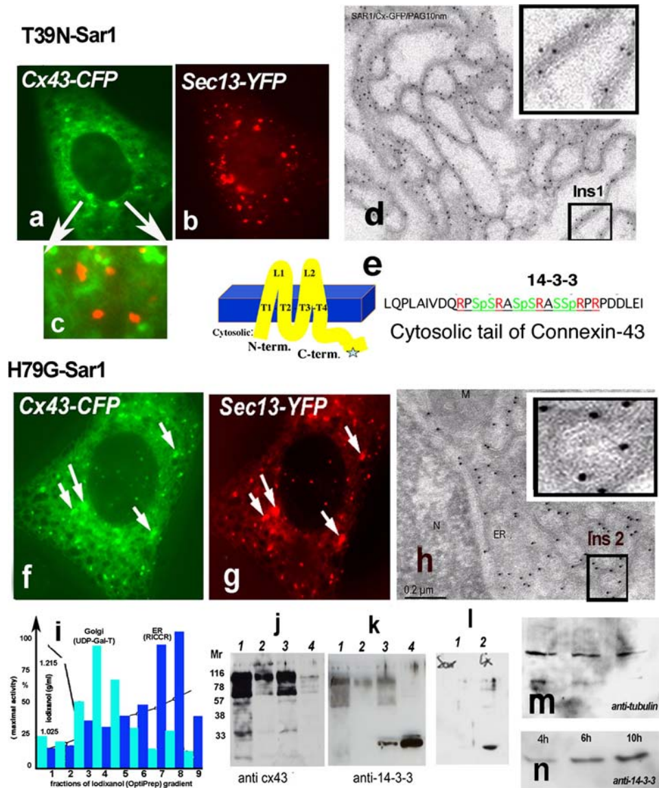
Fig. 2 a–h Two distinct states of Cx43 in the ER in Vero cells expressing Sar1T39N or Sar1H79G. Only Sar1H79G accumulates Cx43 in ER exit sites (ERES) (h). This state correlates with accumulation of 14-3-3 molecules in the ER fraction (see k). a–c Cx43-GFP in cells co-transfected with Sar1T39N remains in the ER membranes, does not segregate into exit sites and does not co-localize with the COPII coat (c, overlay). d Immuno-EM analysis of ultrathin cryosections of Vero cells co-transfected with Cx43-GFP and Sar1T39N probed with anti-GFP antibodies and protein A-10 nm gold revealed that Cx43 immunoreactivity was distributed evenly along an extended ER network and not concentrated in the characteristically rounded ERES. A region of interest ( Ins 1 ) is shown enlarged. e Cx43 transmembrane topology and acid sequence at the cytosolic C-terminus of Cx43 harboring serines in a context suitable for phosphorylation, 14-3-3 protein interaction and RPR/COPI binding motifs. f–g Sar1H79G induces colocalization of Cx43 with the Sec13 subunit of the COPII coat. h Tokuyasu cryo-sections of Vero cells co-transfected with Cx43-GFP and Sar1H79G. Immunogold staining with anti-GFP antibodies show ER cisternae and clearly detectable rounded ERES structures that are decorated with Cx43-GFP. A region of interest showing Cx43 concentrated in ERES is shown ( Ins 2 ). Co-localization between Cx43 and the COPII subunit Sec13-YFP is
