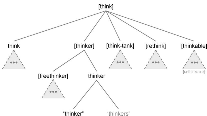
Fig. 3. Morphological paradigms for the polymorphemic word “thinkers”.
