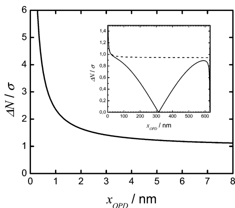
Figure 12. Calculated signal-to-noise ratio as a function of x_{\text{OPD}} according to eq 5 (dashed line: approximation). The signal-to-noise ratio becomes significantly greater than one for values of x_{\text{OPD}} smaller than 2 nm only. The parameters for the shown curves are x_n = 3 nm, N_0 = 1000 , and \lambda = 632 nm.
