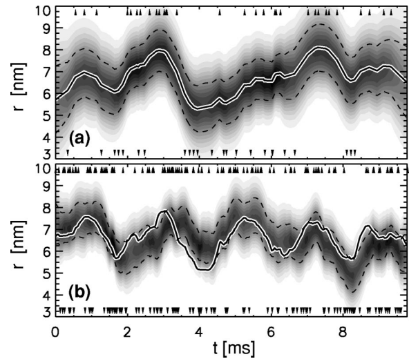
FIG. 3. (a) Distance distribution for a reduced set of 58 photons (wedges) and D = 0.2 \times 10^{-14} m 2 /s; notation as in Fig. 2. (b) Recalculated distance distribution (gray-shaded) for a hypothetical set of 230 photons (wedges) that has been calculated from the original average trajectory in Fig. 2(c), also shown in bold here; D = 0.2 \times 10^{-14} m 2 /s. The dashed lines denote the 1\sigma interval for the recalculated distance distribution.
