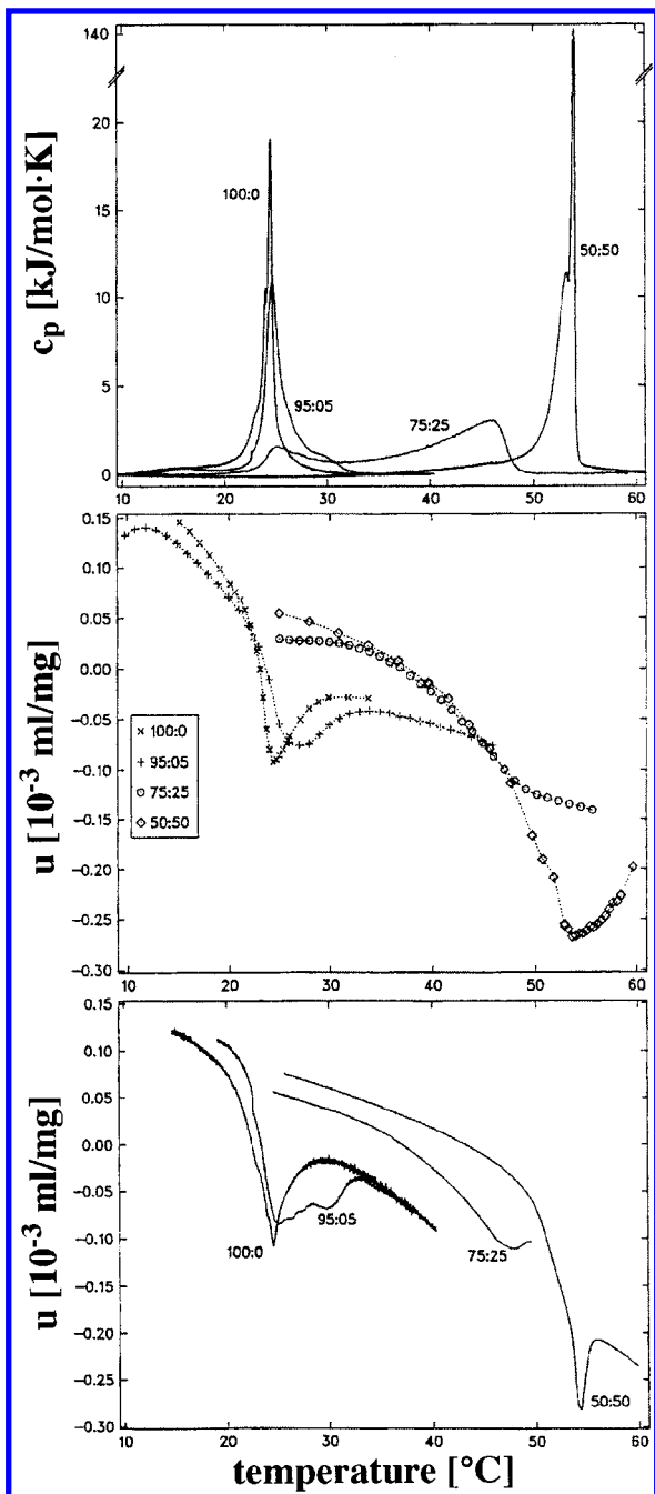
Figure 4. Same plots as Figure 1 but for mixtures of DMPC and DMG.
