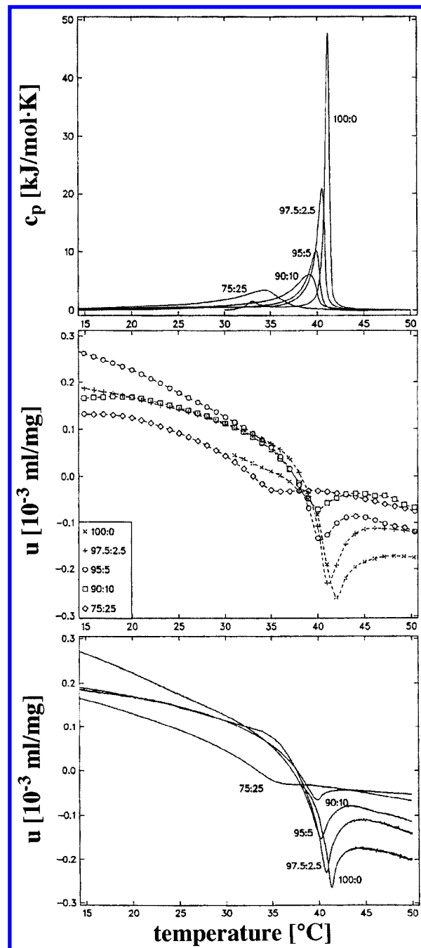
Figure 3. Same plots as Figure 1 but for mixtures of DOPC and DPPC.
