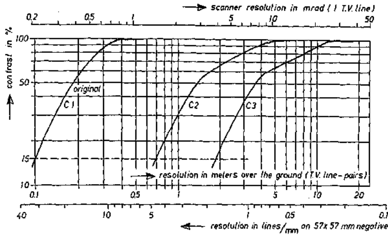
FIG. 4. Modulation Transfer Function of total system.
