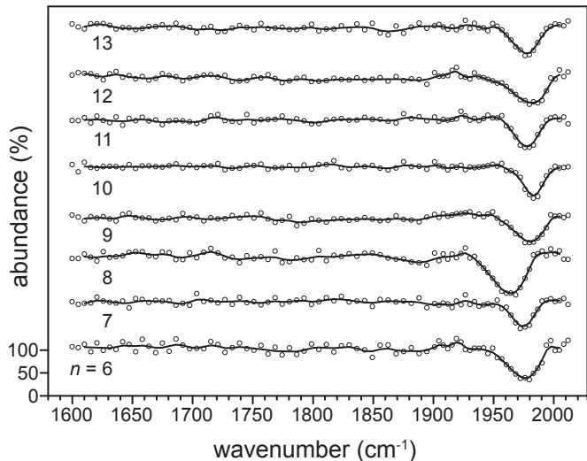
Fig. 1. IR-MPD spectra of CO adsorbed on neutral Ir clusters of different size n . The dots are the actual data points, the line is a binomially weighted five point average.
