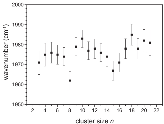
Fig. 2. Peak position of the \nu(\text{CO}) band for different cluster sizes n . The error stems from two parts: an uncertainty in the wavelength calibration of about 0.2 % that equally applies to all values (thus not changing relative peak positions) and the standard deviation of the least square fit to a Gaussian line shape function used to determine the peak positions ( \leq 2.5 \text{ cm}^{-1} ).
