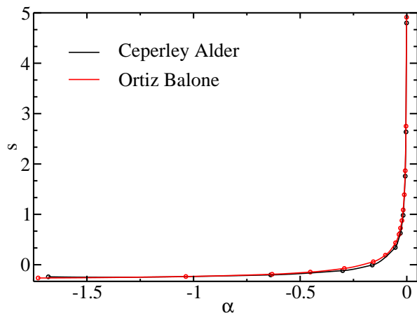
FIG. 1: Dependence of the fitting parameter s of the s -functional 28 on the ratio \alpha of the correlation over the kinetic energy for the HEG. Two different functions s are plotted for two sets of diffusion Monte-Carlo data which s was fitted to reproduce: From Ceperley and Alder 29 and Ortiz and Balone 30 .
