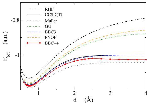
FIG. 2: Dissociation curve of the H 2 molecule with different functionals of the 1-RDM.
