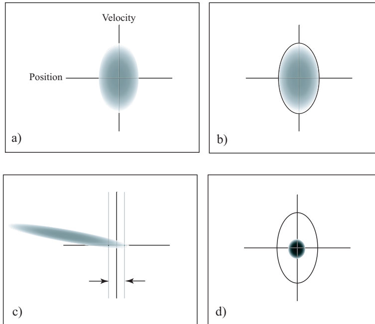
Fig. 4. Idealized longitudinal phase-space distribution at the exit of the decelerator (panel a)) with a perfectly matched acceptance of a trap (panel b)). A spatially elongated, but velocity compressed, longitudinal phase-space distribution (panel c)) that can be transferred to the trap by a spatially localized laser, resulting in an increased phase-space density in the trap (panel d)).
