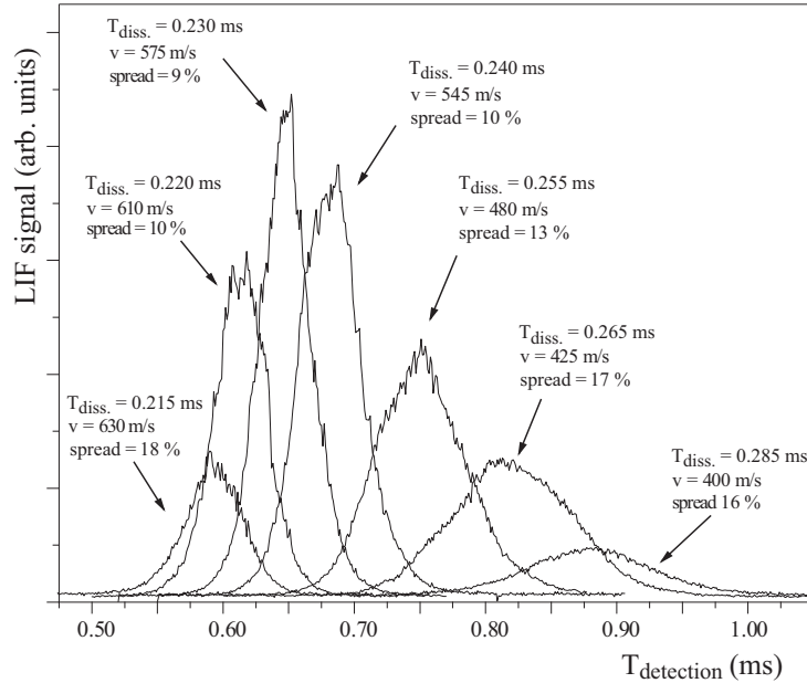
Fig. 2. TOF profiles of the molecular beam of \text{NH} ( a^1\Delta , J = 2 ) radicals for different values of T_{diss} , the time-interval between the trigger for the pulsed valve and the firing of the dissociation laser. For each TOF profile, the mean velocity and the velocity spread (FWHM) of the beam is given.
