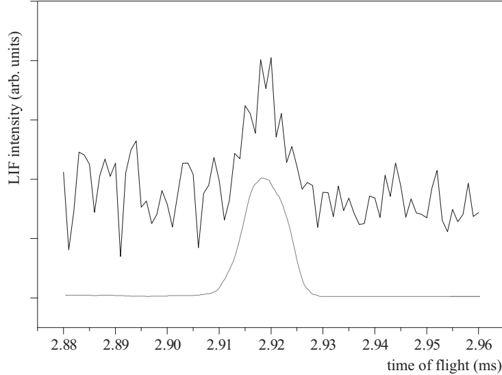
Fig. 3. Observed TOF profile of decelerated NH ( a^1\Delta , J = 2 , M\Omega = -4 ) radicals exiting the decelerator (upper curve). The packet of molecules is decelerated from 550 m/s to 330 m/s. The TOF profile that results from a 3D numerical simulation of the experiment is shown underneath the experimental profile.
