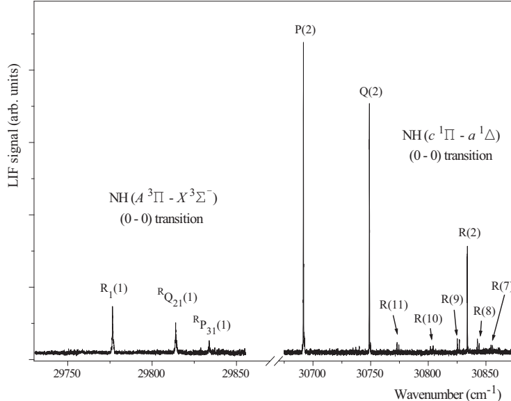
Fig. 1. Fluorescence excitation spectrum of the A^3\Pi, v=0 \leftarrow X^3\Sigma^-, v=0 band and the c^1\Pi, v=0 \leftarrow a^1\Delta, v=0 band of NH in the pulsed molecular beam. The lines are labelled using standard spectroscopic nomenclature.
