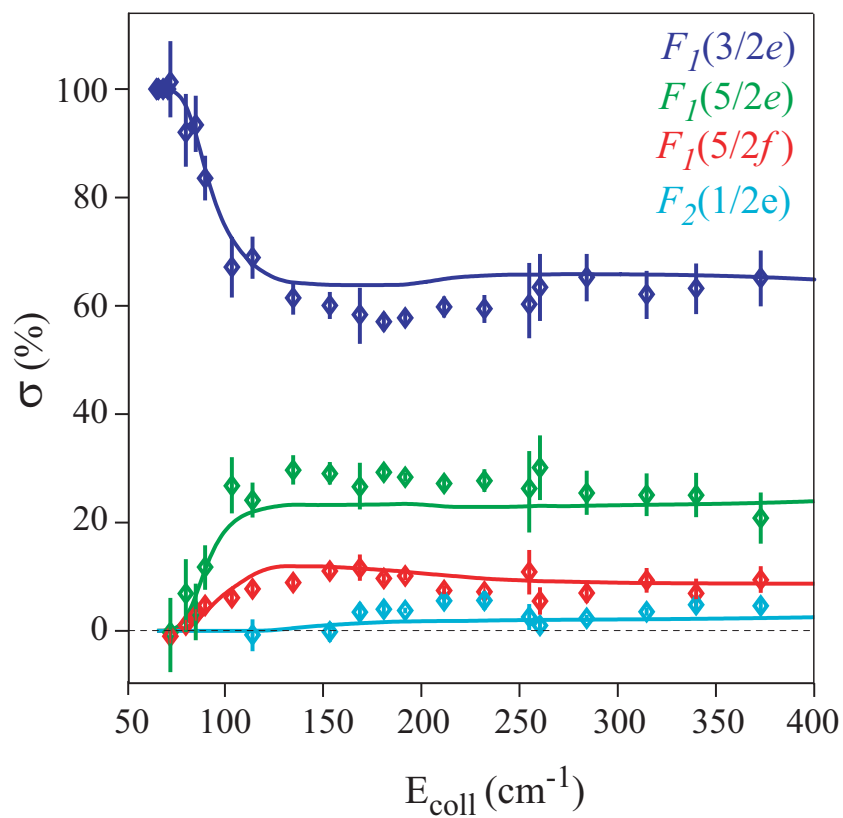
Figure 4: Comparison of the collision energy dependence of the measured (data points with error bars) and calculated (solid curves) relative cross-sections - i.e., the fractional scattering of OH radicals into one of the F_1(3/2e) , F_1(5/2e) , F_1(5/2f) , or F_2(1/2e) channels.
