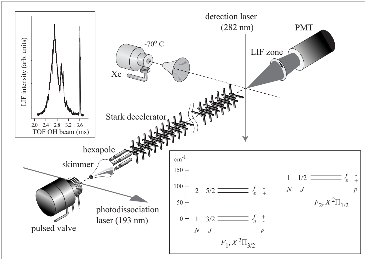
Figure 1: Schematic representation of the experimental setup and of the energy-level scheme of the OH radical. The OH radical beam is produced by photodissociation of gaseous \text{HNO}_3 that is coexpanded with a noble carrier gas (Ar, Kr, or Xe) into a vacuum. The beam is skimmed and radicals in the low-field-seeking F_1(3/2_f) state are focused with a hexapole into the Stark decelerator, where the beam is decelerated, guided or accelerated to a velocity in the 33 to 700 m/s range. A typical time-of-flight (TOF) profile is shown in the left inset. The selected packet of radicals arrives temporally separated in the scattering region and is scattered with a beam of pure Xe at an angle of 90^\circ , under single-collision conditions. The collision-induced populations in the F_2(1/2) , F_1(3/2) , and F_1(5/2) rotational levels are probed before and after the collisions using a pulsed dye laser system in a saturated laser induced fluorescence (LIF) scheme. The fluorescence is imaged onto a photomultiplier tube (PMT). In the energy-level scheme shown in the right inset, the splitting between both parity components of each rotational level is largely exaggerated for reasons of clarity.
