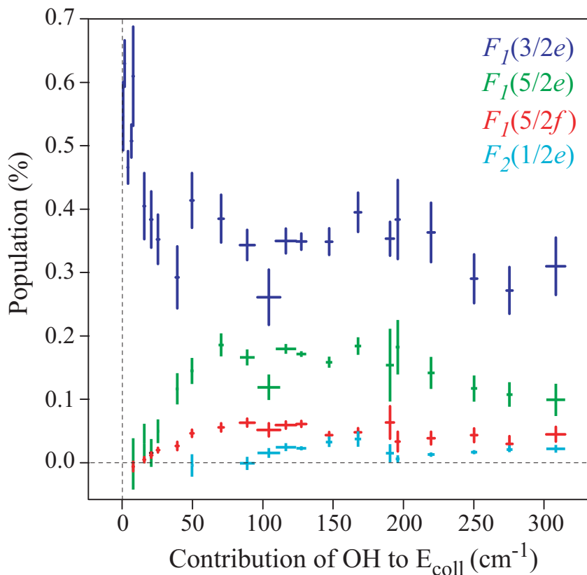
Figure 2: Probabilities for inelastic scattering of OH F_1(3/2f) radicals in collisions with Xe atoms to the F_1(3/2e) , F_1(5/2e) , F_1(5/2f) , and the F_2(1/2e) levels as a function of \frac{1}{2}(\frac{m_{OH}m_{Xe}}{m_{OH}+m_{Xe}})v_{OH}^2 - i.e., as a function of the contribution of OH to the CM collision energy (where m_{OH} and m_{Xe} are the mass of OH and Xe, respectively, and v_{OH} is the velocity of the OH radicals in the laboratory frame). The horizontal error bars represent the uncertainty in collision energy that results from the velocity spread of the OH beam, which is different for every setting of the decelerator. The vertical error bars represent the statistical spread of the data as obtained from repeated runs of the experiment.
