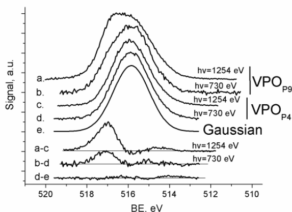
Figure 4: Comparison of V2p_{3/2} peaks of VPO_{p4} and VPO_{p9} at reaction conditions. a-b) VPO_{p9} , c-d) VPO_{p4} , e) Gaussian
