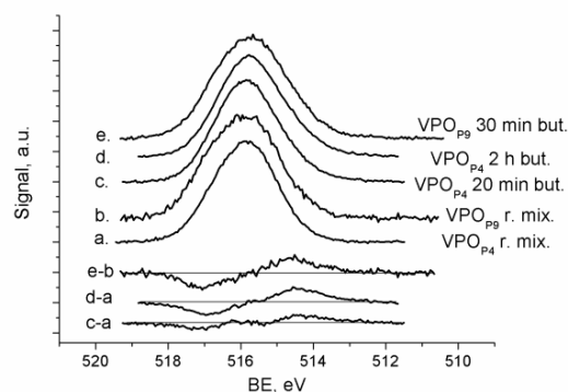
Figure 5: Changes of surface V2p_{3/2} spectra in n -butane at 400°C. a) VPO_{p4} in reaction mixture, b) VPO_{p9} in reaction mixture, c) VPO_{p4} after 20 min in n -butane, d) VPO_{p4} after 2 hours in n -butane, e) VPO_{p9} after 30 min in n -butane
