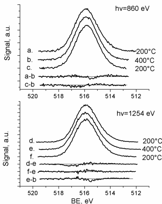
Figure 2: V2p 3/2 spectra of VPO P4 in heating-cooling experiment. a-c) hv=860 eV, d-f) hv=1254 eV
