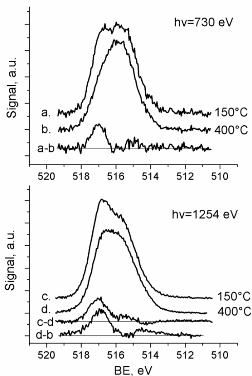
Figure 3: V2p_{3/2} spectra of VPO_{p9} before and after heating in reaction mixture. a-b) h\nu=730 eV, c-d) h\nu=1254 eV
