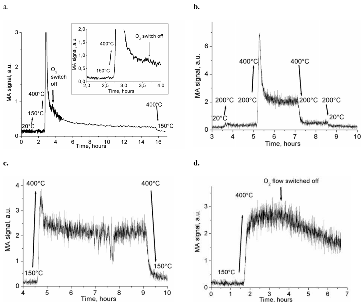
Figure 1: Catalytic reactivity towards MA registered by PTRMS (signal on m/e=99 amu/e). a) VPO p0 in reaction mixture and in n -butane/He atmosphere, b) VPO p4 in reaction mixture- first heating, c) second heating, d) third heating and in n -butane/He atmosphere
