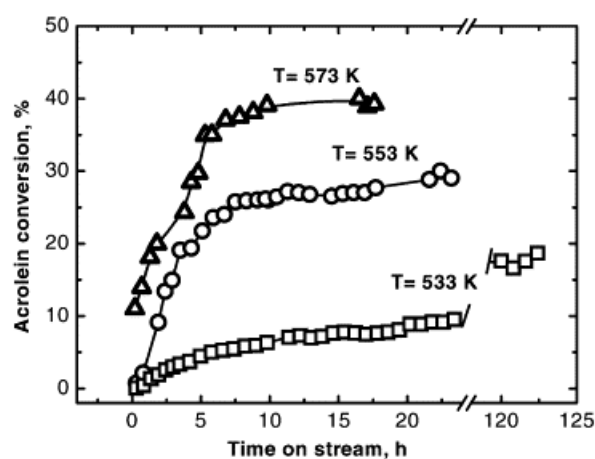
Fig. 1. Acrolein conversion over the Mo 9 V 3 W 1.2 O x catalyst at 533 K (open squares), 553 K (open circles), and 573 K (open, bold triangles) and \dot{V} = 0.04 g s/ml as a function of operation time on stream. Reaction mixture composition: 4% C 3 H 4 O, 10% O 2 , 20% H 2 O, balance He.
