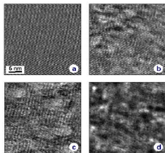
Figure 3: High-resolution images of V_2O_5 during irradiation. Irradiation times: a: 0 min; b: 7 min; c: 10 min; d: 15 min. The V_2O_5 specimen is oriented slightly off the 001 axis.
