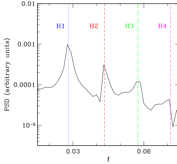
Figure 4. Power spectral density of the evolution of the central rest-mass density for the model closest to the putative critical solution (i.e. with \rho_c = 0.004\,593\,224\,8034 ) when the secular drift part (15) has been removed from the data. The eigenfrequencies associated with the corresponding spherical star model are also shown as vertical lines.
