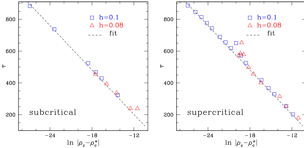
Figure 5. Escape time \tau as a function of \ln |\rho - \rho^*| for subcritical (left panel) and supercritical solutions (right panel), respectively. The blue squares correspond to the results obtained with the h = 0.1 resolution, while the red triangles to the results obtained with the h = 0.08 resolution. The dashed lines represent the fit obtained using equation (17) with \lambda obtained from the h = 0.1 solutions.
