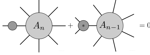
Figure 1. Deformed superconformal invariance relation for tree amplitudes.
