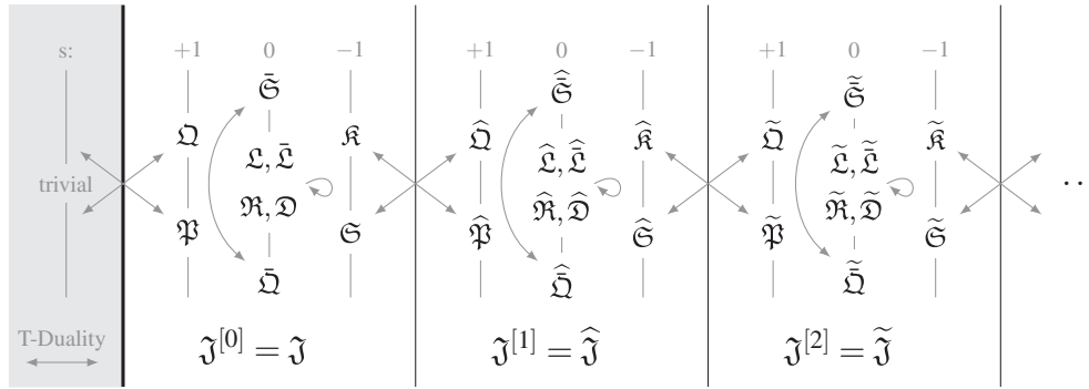
Figure 6. The level- r Yangian generators map under T-duality ( \rightarrow ) to different levels according to their weight s = \pm 1, 0 under the sum of the dilatation generator \mathcal{D} and the hypercharge \mathcal{B} of \mathfrak{su}(2, 2|4) .
