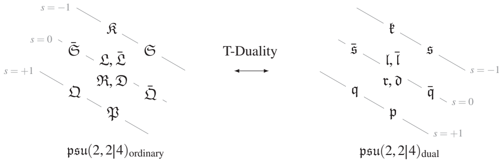
Figure 5. The ordinary representation of the superconformal algebra and its dual symmetry. The lines of constant eigenvalue under the commutator with the sum of the dilatation generator and the hypercharge of \mathfrak{psu}(2, 2|4) are indicated in gray.
