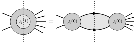
Figure 3. Essential contribution to the one-loop unitarity cut.
