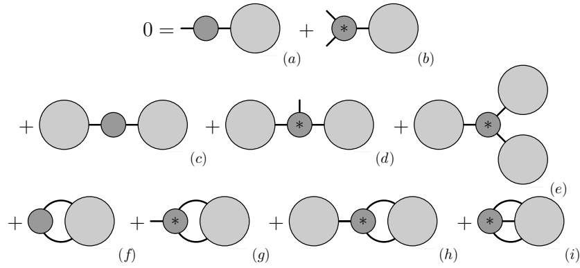
Figure 2. General superconformal invariance relation (qualitatively). Terms (a) and (b) correspond to figure 1, terms (c)–(e) are needed for factorized amplitudes, and terms (f)–(i) are needed for loops. A big circle represents a connected scattering amplitude. A small circle represents a free conformal generator (empty) or the three-point kernel (starred).
