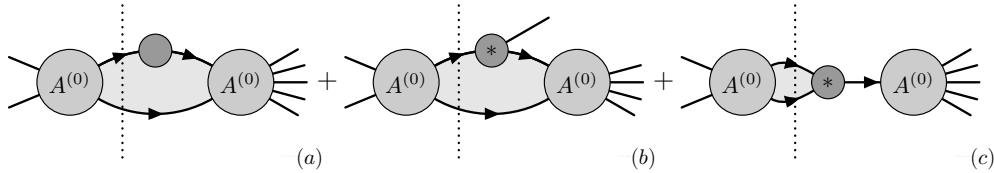
Figure 4. Essential contributions to the one-loop superconformal variation.
