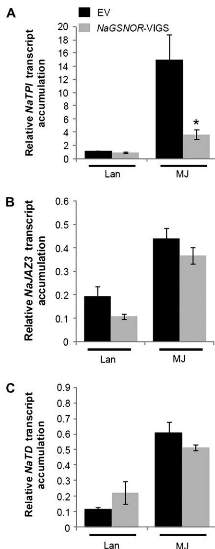
Fig. 8. Transcript levels of NaTPI , NaJAZ3 , and NaTD in methyl jasmonate-treated EV and NaGSNOR -VIGS plants. EV and NaGSNOR -VIGS plants were applied with lanolin pastes (20 \mu l) containing 5 mg ml -1 methyl jasmonate (MJ), or pastes of pure lanolin (Lan) (20 \mu l) for comparison. The transcript levels of NaTPI (A), NaJAZ3 (B), and NaTD (C) (mean \pm SE) were determined in EV and NaGSNOR -VIGS plants 8 h after treatments. Stars indicate significantly different levels between EV and NaGSNOR -VIGS plants (Student's t test; * P \leq 0.05; n = 5).
