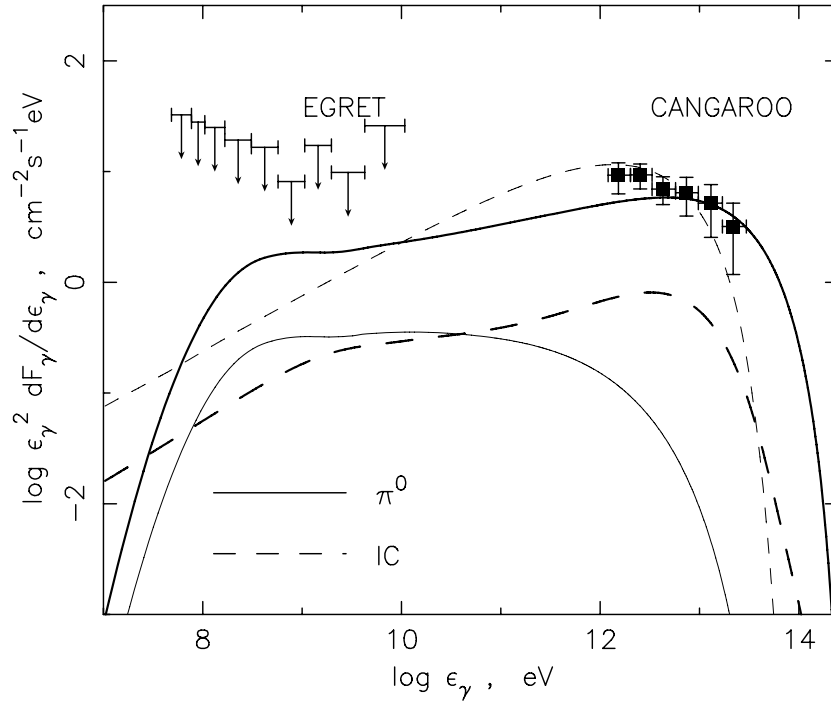
Fig. 5. Theoretical IC ( dashed lines ) and \pi^0 -decay ( solid lines ) \gamma -ray spectral energy densities for SN 1006. Efficient proton acceleration is indicated by the thick curves, inefficient proton acceleration by the thin curves. The recent high energy \gamma -ray flux data and the EGRET upper limits [48] are also shown (from [18])
