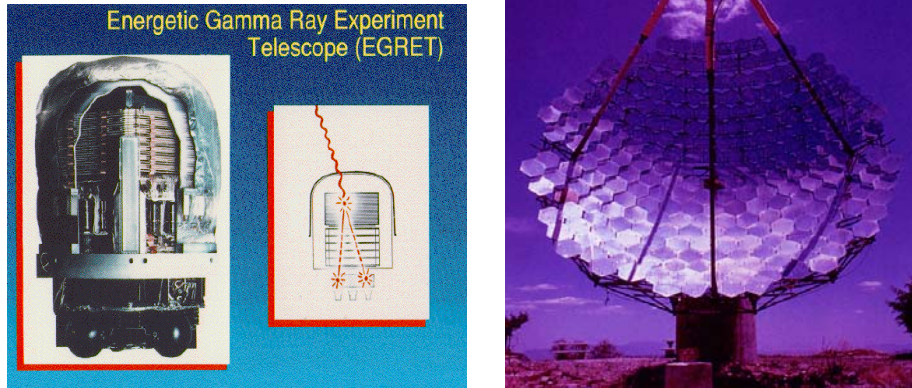
Fig. 1. (Left) The EGRET instrument on the Compton Gamma Ray Observatory (CGRO). Left: overall instrument with anti-coincidence shield. Right: schematic of conversion of the incoming primary \gamma -ray into an e^+e^- pair that is tracked in a spark chamber, with energy measurement in the calorimeter on the bottom
