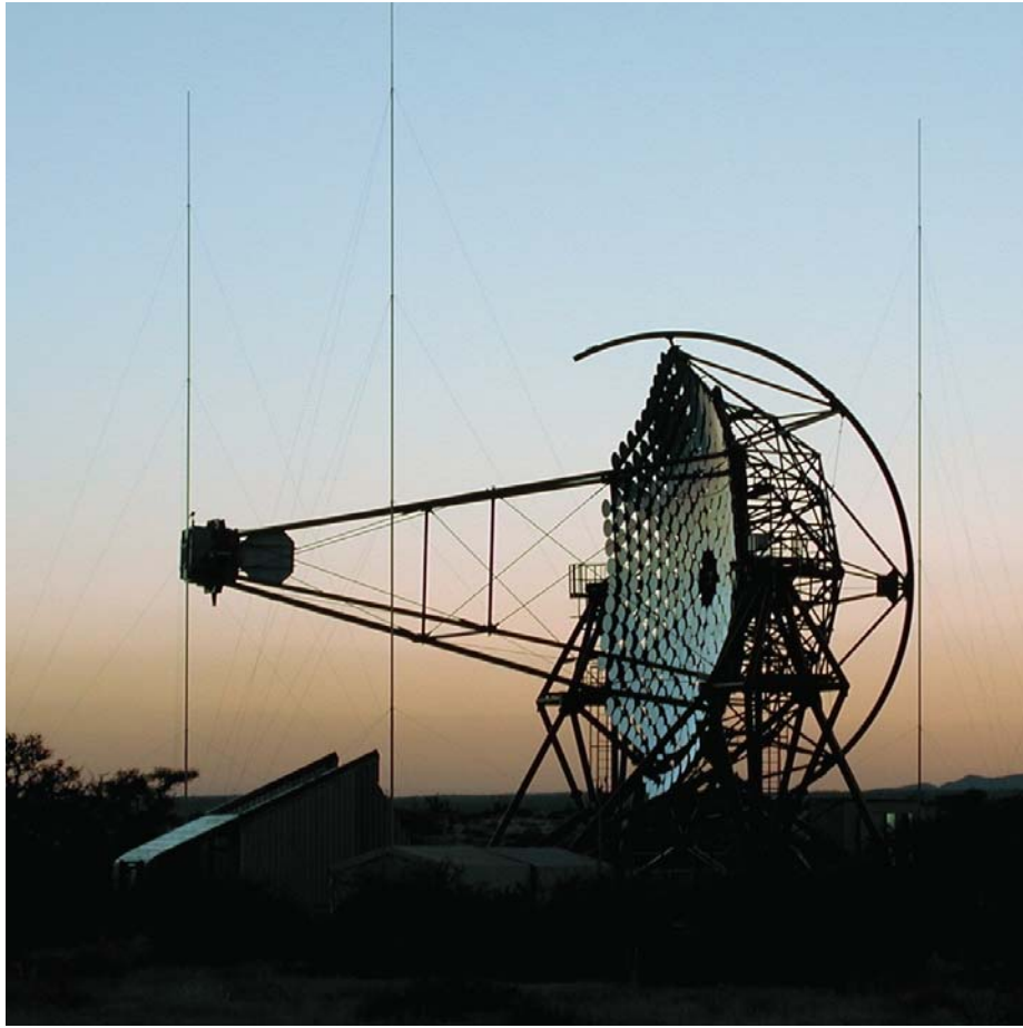
Fig. 11. The first of the four 12 m telescopes of H.E.S.S. Phase I in Namibia. The tessellated mirror consists of 380 aluminized glass mirrors of 60 cm diameter. The focal plane detector ('camera') has 960 ultrafast photomultiplier pixels, covering an area of 1.4 m that corresponds to a field of view of 5^\circ . The energy threshold is about 100 GeV and the sensitivity is about 10^{-12} erg/(cm 2 s) above 100 GeV and about 10^{-13} erg/(cm 2 s) above 1 TeV for 50 h of observation. (Photograph F. Toussenel, June 2002)
