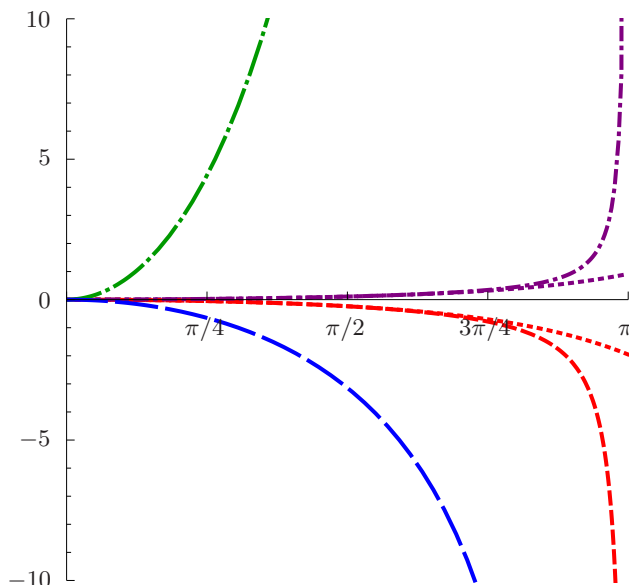
Figure 3. Curves showing V^{(1)}(\phi, 0) (blue, wide dashes), V^{(2)}(\phi, 0) (green, dash-dot), V_{\text{AdS}}^{(0)}(\phi, 0) (red, short dashes) And V_{\text{AdS}}^{(1)}(\phi, 0) (purple, short dash-dot). Note that all have a simple pole at \phi = \pi , with different residues. The dotted lines show the perturbative expansions of V_{\text{AdS}}^{(0)} and V_{\text{AdS}}^{(1)} around \phi = 0 to order \phi^8 , (6.5), (6.6), which furnish a good approximation up to \phi \sim 2 .
