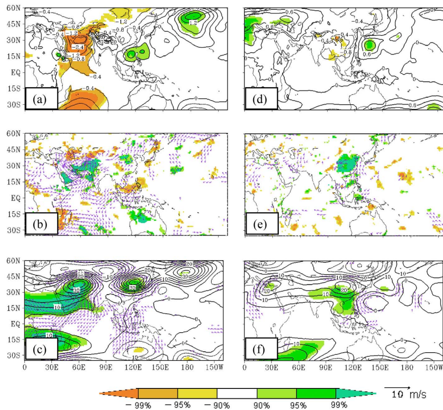
Figure 1. Mean difference of 21 summer seasons (June–September) from 1979–1999 between the intensified and shallow heat low experiment (IMSHL) (a) sea level pressure (hPa) (b) 850 hPa wind (vectors) and surface precipitation (shaded) (c) 200 hPa geopotential height (contours) and wind (vectors). The shaded areas in Figures 1a–1c indicate differences that are significant at 90% confidence level based on t-test for mean sea level pressure, surface precipitation and 200 hPa geopotential height respectively. The wind vectors associated to differences below 95% confidence level are omitted in Figures 1b and 1c. Negative contours in Figures 1a and 1c are shown by dashed line. (d, e) Similar to Figures 1a–1c except for EAIME experiment.
