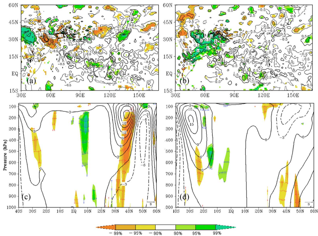
Figure 2. Mean differences of vertical velocity at 500 hPa (a) IHL minus Control experiment (b) SHL minus Control experiment. The difference in the height–latitude cross-section of vertical velocity (shaded) and geopotential height (contours) averaged between 100°–120°E (c) IHL minus Control experiment (d) SHL minus Control experiment. The difference is computed for 21 summer seasons (June–September) from 1979–1999 using monthly data. The shaded areas in Figures 2a–2d indicate differences that are significant at 90% confidence level for vertical velocity based on t-test. The vectors in Figures 2c and 2d indicate ascent (descent) if pointing upward (downward). The blue (red) vectors show significant increase (decrease) in ascent or descent. The wind vectors associated to differences below 90% confidence level are omitted in Figures 2c and 2d. The negative contours in Figures 2a–2d are shown by dashed lines.
