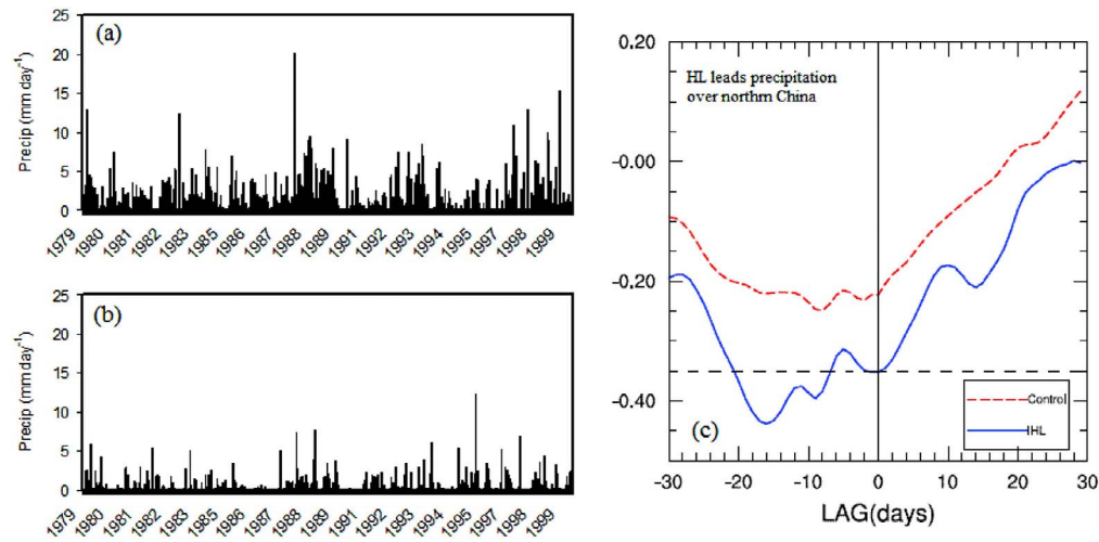
Figure 3. Area averaged daily rainfall over the HL region (a) IHL, (b) SHL. (c) The lead-lag correlations between the sea level pressure over HL region and rainfall over northern China ( 35^{\circ} – 42^{\circ} N, 100^{\circ} – 120^{\circ} E). The solid and dashed line in Figure 3c represents the correlations during the intense HL years and the Control experiment respectively. Out of 21 year 7 years are identified as IHL years. The horizontal dashed line in Figure 3c represents the 95% confidence level for correlations using the t-test.
