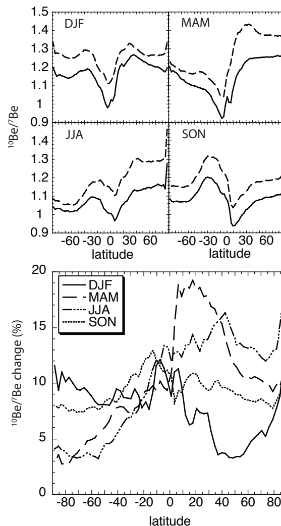
Fig. 11. The seasonal ^{10}\text{Be}/^7\text{Be} ratio of the deposition fluxes (Maunder Minimum: dashed line, Present day: full line), and the difference between Maunder Minimum and Present day in %.
