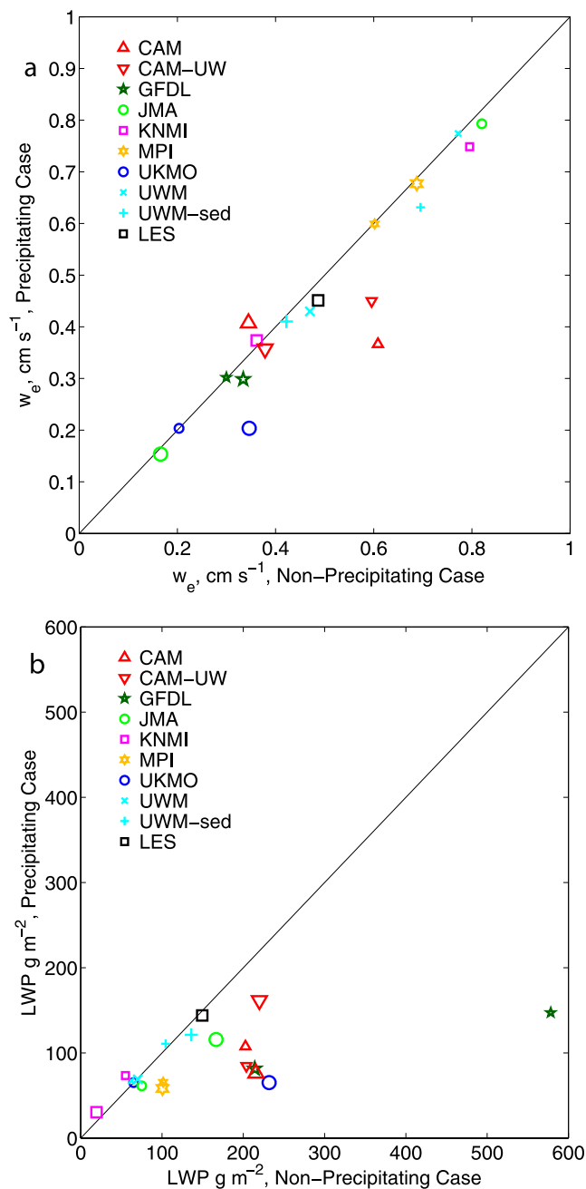
Figure 6. (a) Mean entrainment rate over the final two simulation hours, with symbols as in Figure 3. For the SCMs the larger symbol indicates standard-resolution run and the smaller symbol, when present, indicates the high-resolution run. The thin black line represents no difference between precipitating and nonprecipitating cases. (b) Same as Figure 6a except with liquid water path.
