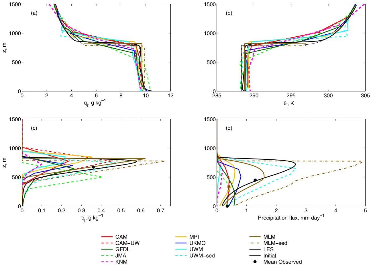
Figure 2. SCM and LES profiles at hour 6 of (a) total specific humidity, q_t ; (b) liquid water potential temperature, \theta_l ; (c) cloud liquid water, q_l ; and (d) precipitation flux. The initial profiles of q_t and \theta_l are plotted as thin black lines. The peak in the mean RF02 q_l profile [vanZanten and Stevens, 2005] and mean observed precipitation flux values at cloud base and at the surface are plotted as black dots [vanZanten et al., 2005].
