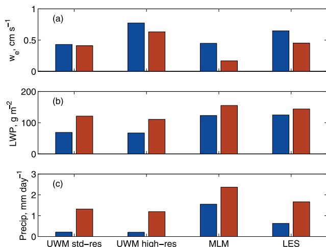
Figure 7. A comparison of runs without (blue) and with (red) droplet sedimentation for four model configurations: UWM at standard resolution, UWM at high resolution, the mixed layer model (MLM), and the DHARMA LES. Plotted are final 2 h averages of (a) entrainment rate, (b) liquid water path, and (c) cloud base precipitation.
