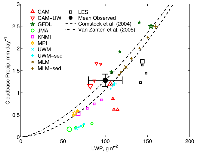
Figure 4. Same as Figure 3 except for high-resolution case. UKMO did not submit a high-resolution simulation. LES and MLM runs are identical to those shown on Figure 3.
