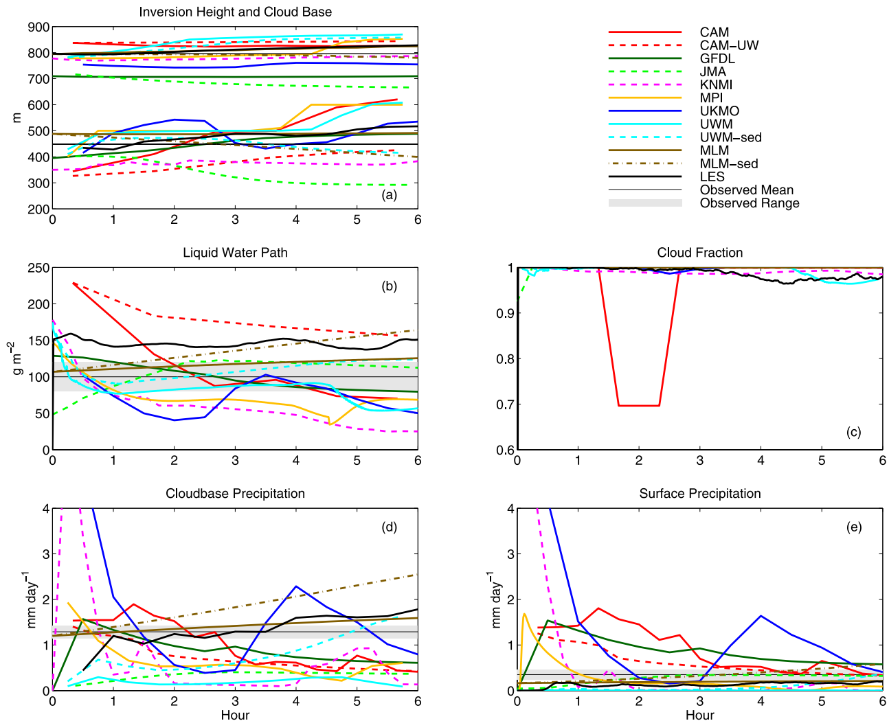
Figure 1. Evolution of (a) inversion height and cloud base, (b) liquid water path, (c) cloud fraction, (d) cloud base precipitation, and (e) surface precipitation for the standard-resolution case. Also plotted is the evolution of DHARMA LES (thick black lines), observed mean values (thin black line) and uncertainty range of observations (gray shading). Observed values of inversion height and cloud base (LCL) are from vanZanten and Stevens [2005], and values of precipitation are from vanZanten et al. [2005].
