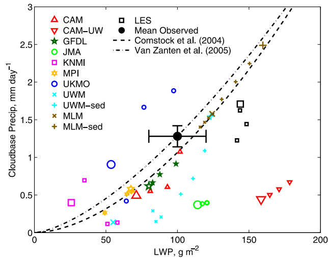
Figure 3. Mean cloud base precipitation and liquid water path for the SCMs at standard resolution, the MLM, and the LES. For each model the large symbol represents the hour 6 mean, and the smaller symbols represent the means for hours 3, 4, and 5. The observed mean RF02 value is plotted with uncertainty bars. Empirical relations between LWP and cloud base precipitation are plotted as dashed and dashed-dotted lines.
