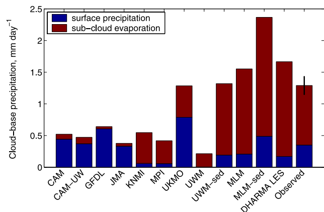
Figure 5. Mean cloud base precipitation rate for the last two simulation hours of the standard case as compared with mean RF02 observations. This rate is partitioned into mean surface precipitation rate (blue) and the subcloud evaporation rate (red). Uncertainty in observed cloud base precipitation is plotted as a black line.
