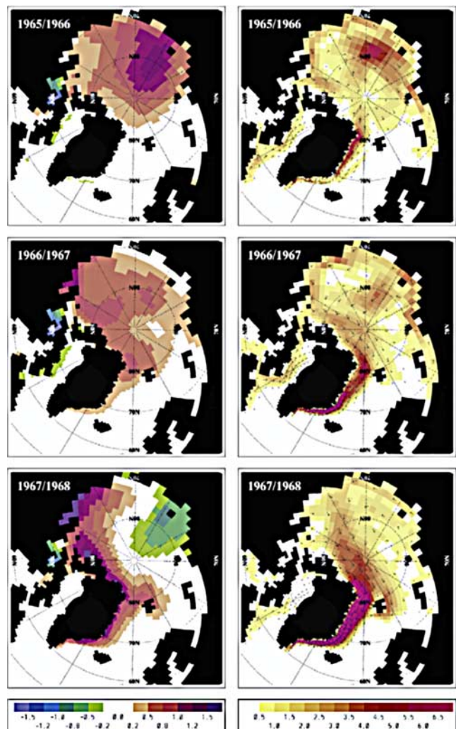
Figure 2. Ensemble mean sea ice thickness anomaly (left column) and sea ice transport anomaly (right column, every forth vector plotted) for the years 1965/66, 1966/67 and 1967/68. Shown are annual mean values centered on winter. Units are m and 10^{-2} \text{ m}^2/\text{s} , respectively.
